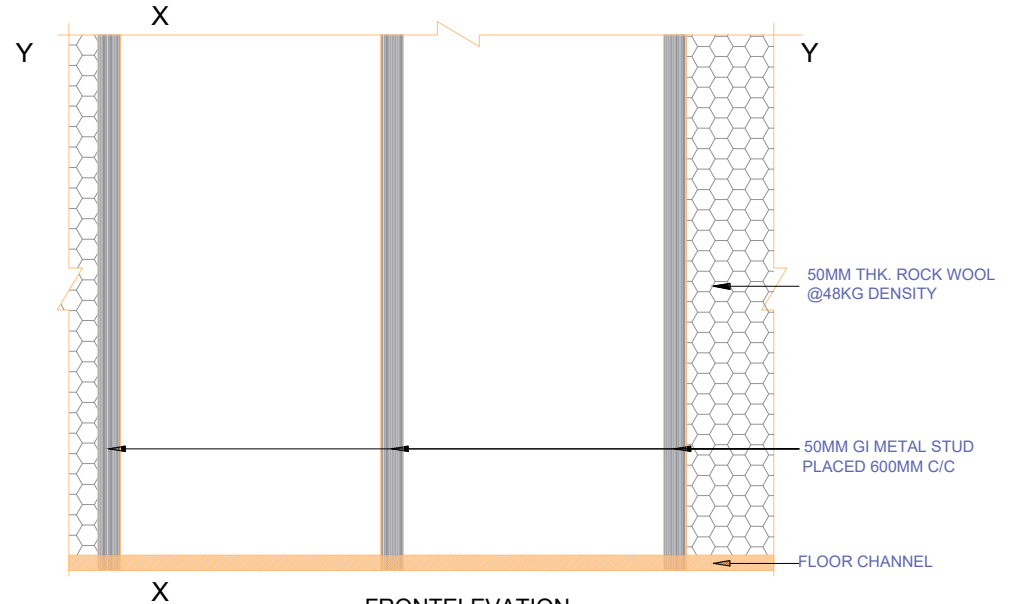
FRONT ELEVATION DETAIL OF WALL
